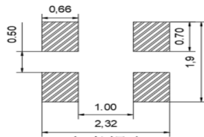
参考焊盘 Reference Soldering Pad
