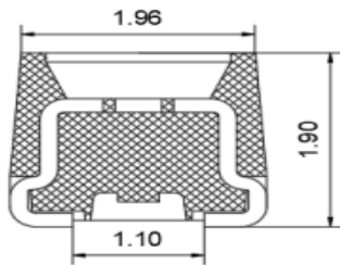
剖面图 Cutaway view
