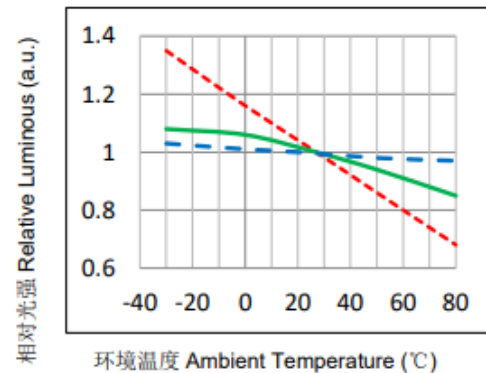
Ambient Temperature VS. Relative Luminous
