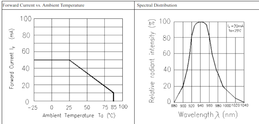
Typical Electrical/Optical/Characteristics Curves for IR
