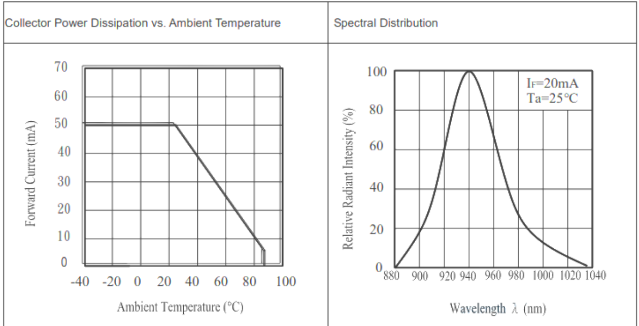
Typical Electrical/Optical/Characteristics Curves for IR
