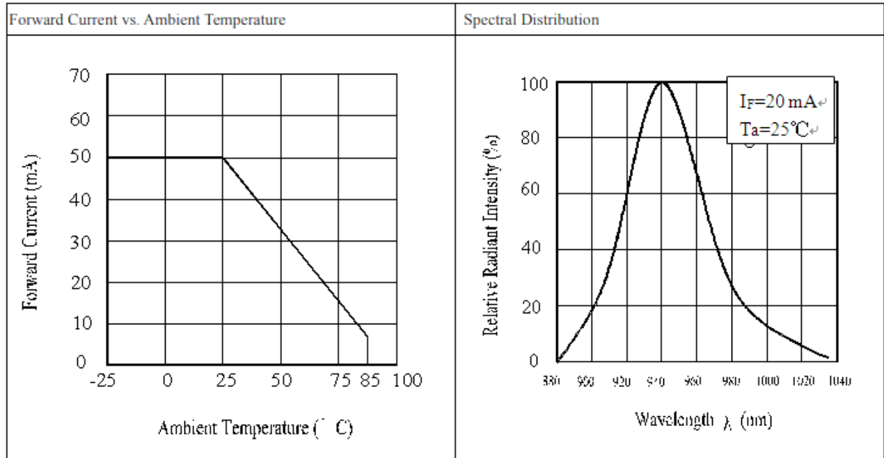
Typical Electrical/Optical/Characteristics Curves for IR
